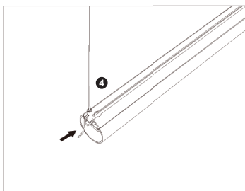
4. Install the suspension kits
