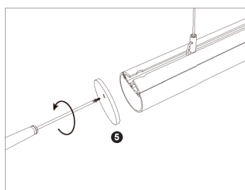
5. Screws the end caps
